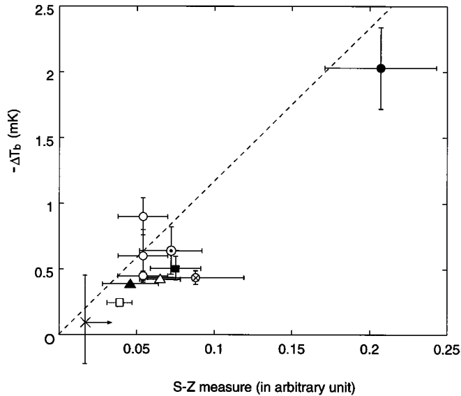
FIG. 3.—Observed S-Z decrement vs. S-Z measure, R_C^{-0.5} f(T) , together with the theoretical one (dashed line). The sources are A401 (circled dot), A478 (filled triangle), A665 (circled cross), A1204 (cross; present result), A1656 (filled square), A2142 (open triangle), A2163 (filled circle), A2218 (open circles), and A2256 (open square). Data are from Rephaeli (1995), Herbig et al. (1995), Jones (1994), and Furuzawa et al. (1994). Values of \Delta T_b obtained from observations at different frequencies have been converted to the value at 15 GHz.
