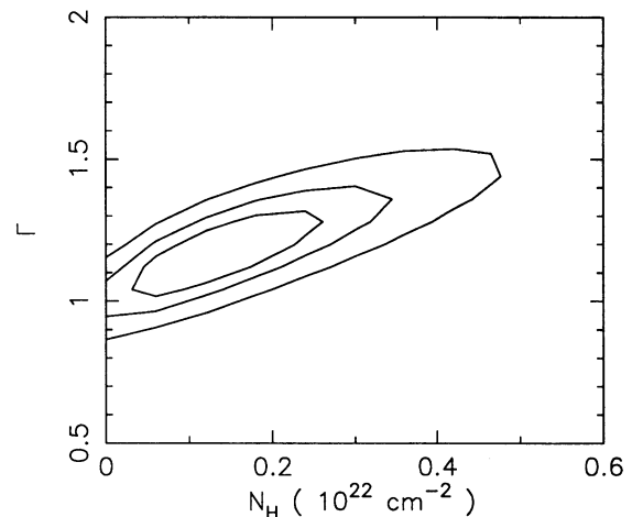
FIG. 3.—Confidence contours of photon index ( \Gamma ) vs. column density ( N_H ) for the four-instrument spectral fit with a simple power-law-plus-absorber model. The confidence levels are 68%, 90%, and 99% for two interesting parameters.
