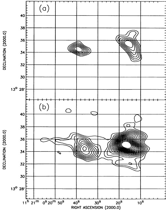
FIG. 1.— ASCA S3 image of NGC 3628 (a) below 2 keV and (b) above 2 keV, smoothed with a \sigma \sim 30'' Gaussian (without background subtraction). The contours correspond to levels of 0.45–1.35 smoothed counts at intervals of 0.1 smoothed counts.
